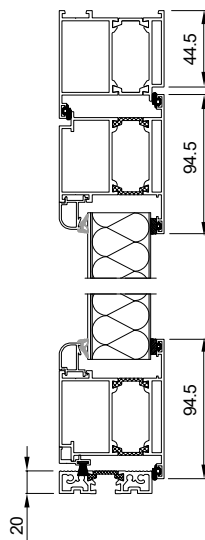
DoorTherm 86 Profile Dimensions
